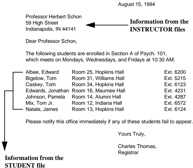
Figure 1-4. Class List
