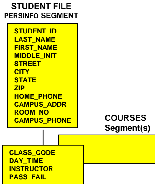
Figure 1-3. Student File
